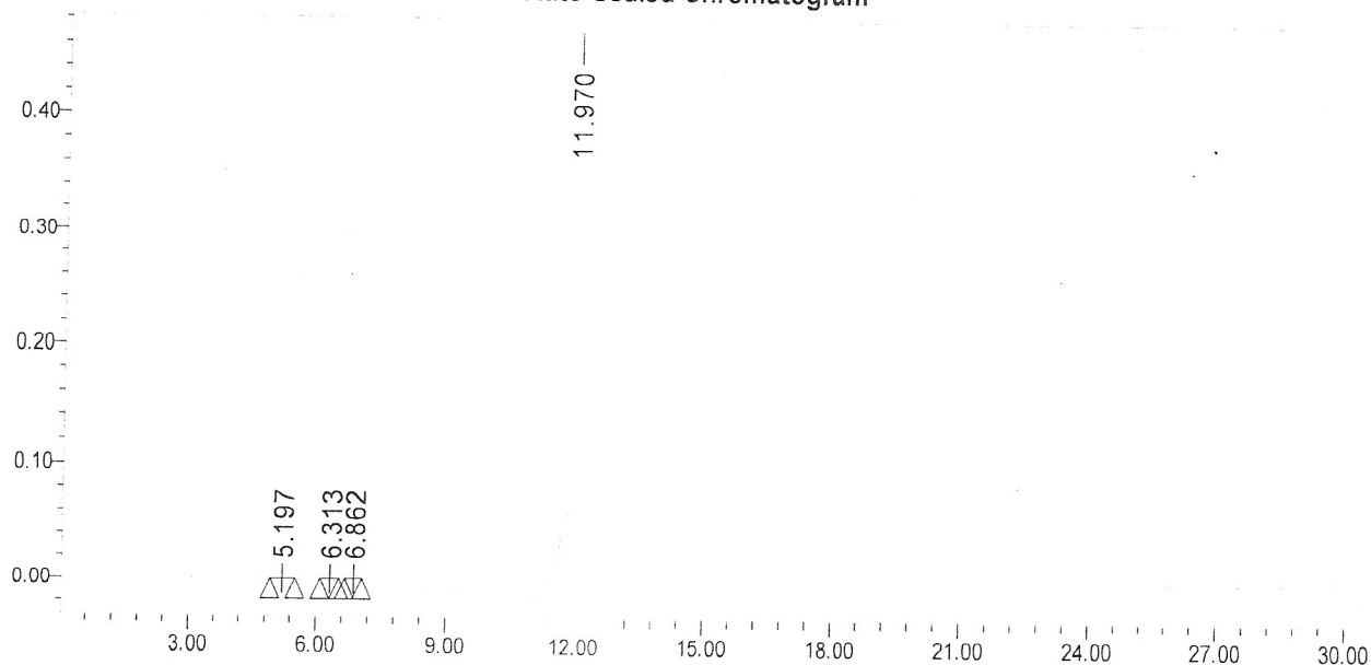
Auto-Scaled Chromatogram
